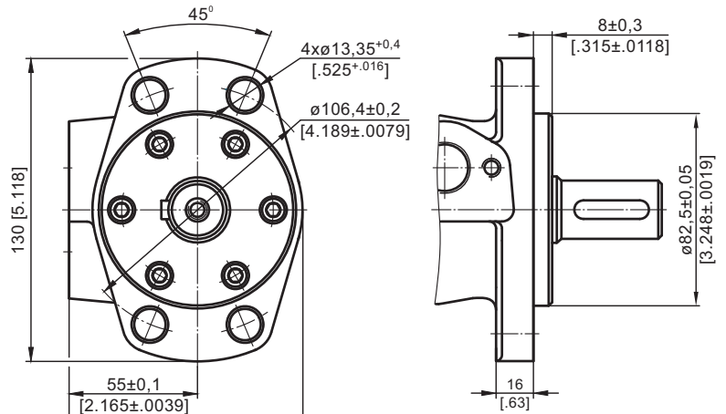
F - Oval mount (four holes)
